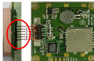
Fig2. PIN Header
