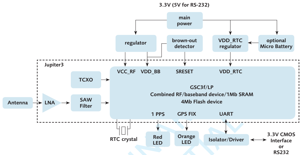
Figure 2-1: Receiver architecture
