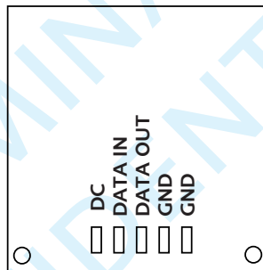
Figure 4-1: Electrical Connections view from solder side
