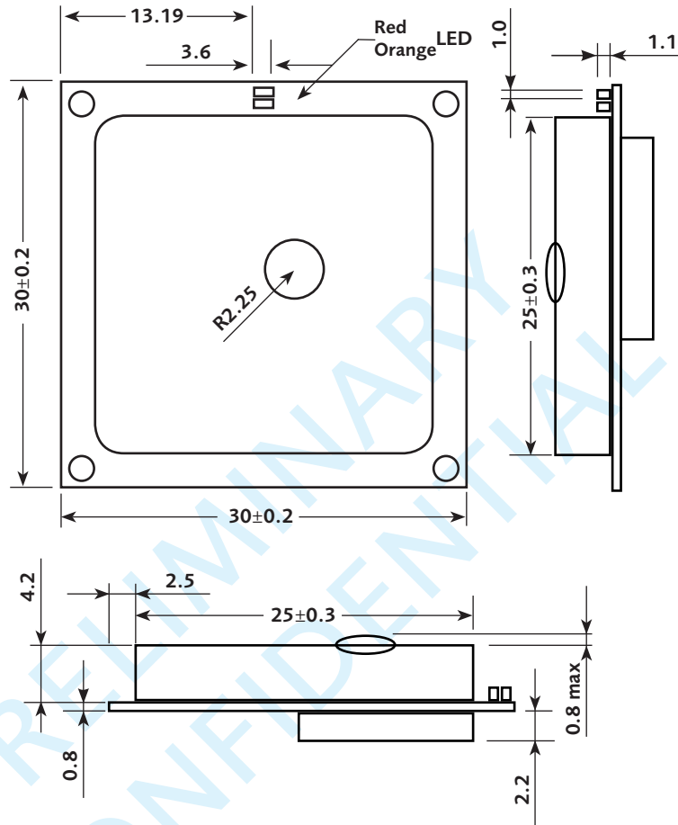
Figure 2-2: Antenna: Physical dimensions
