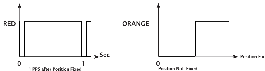
Figure 3-1a: Optional LED indicator duty cycle for TTL Version
