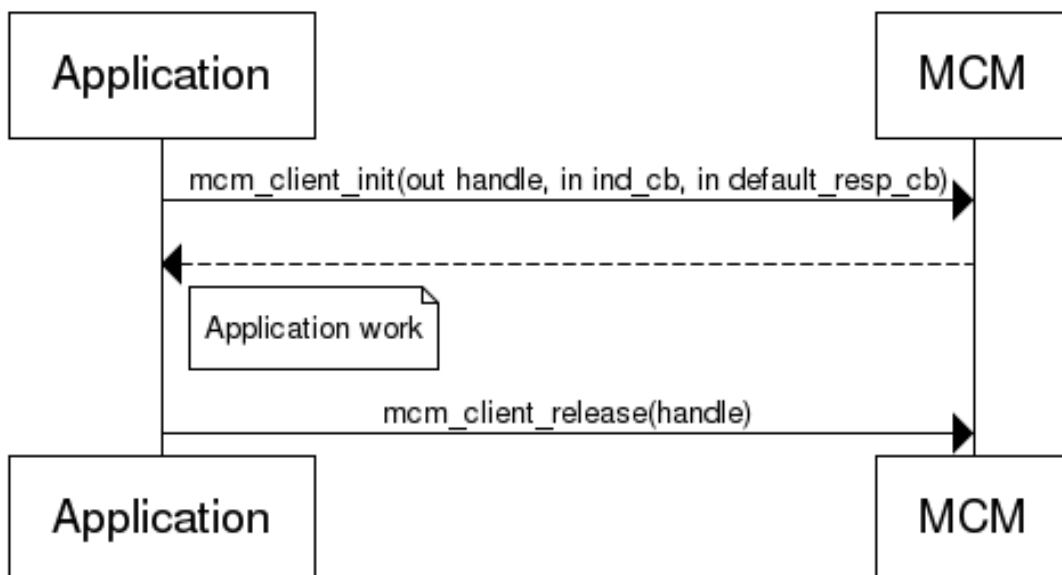
Figure 2-1 Client initialization and release call flow
