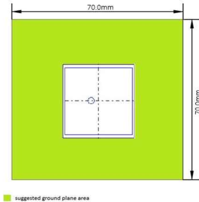
Figure Error! No text of specified style in document.-7 Recommended Ground Plane
