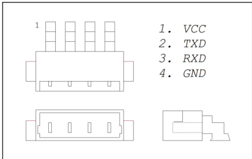
Figure Error! No text of specified style in document.-5 SC872-A Module Pinout
