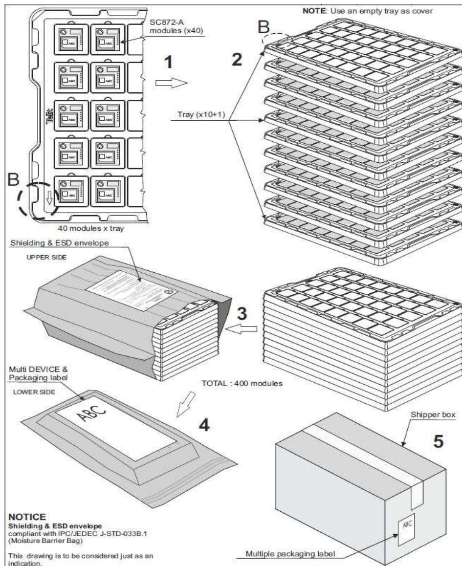
Figure Error! No text of specified style in document.-10 Tray Packaging
