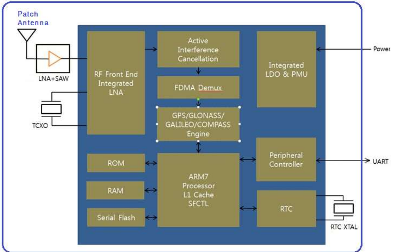
Figure Error! No text of specified style in document.-1 SC872-A Block Diagram
