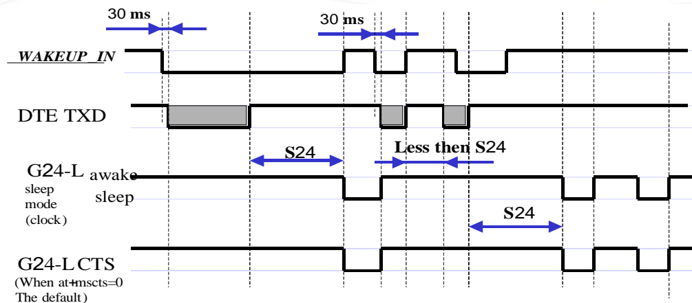
Figure 4-11: Sleep Mode when S24 > 0
