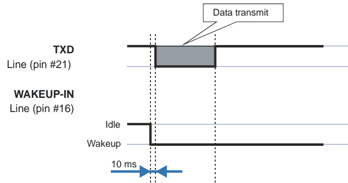
Figure 3-9: Wakeup-In Line
