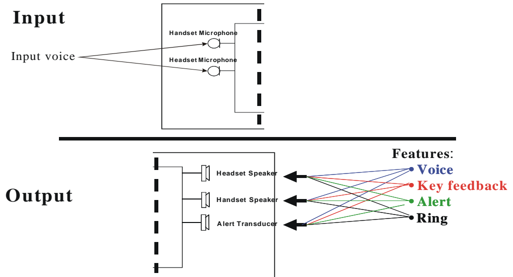
Figure 3-6: Audio Paths
