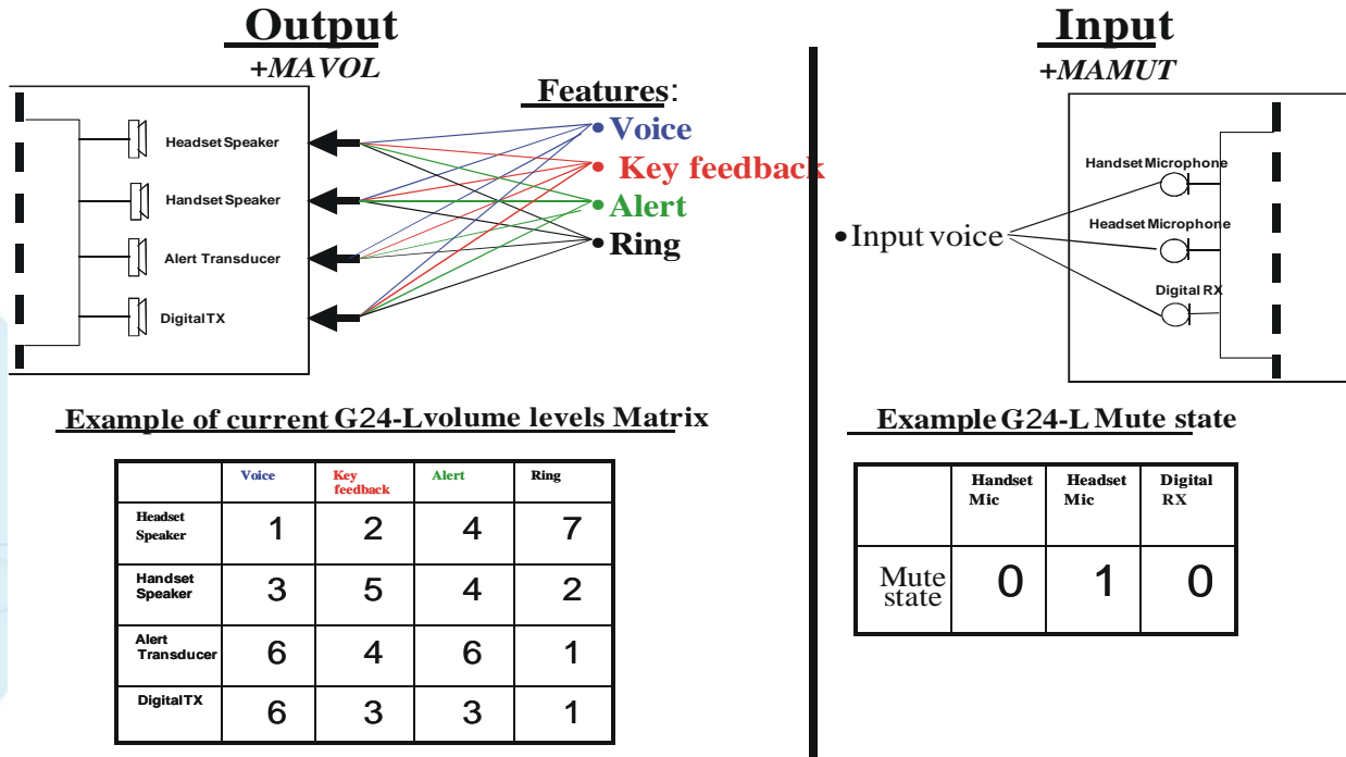
Figure 3-7: G24-L Audio Gain
