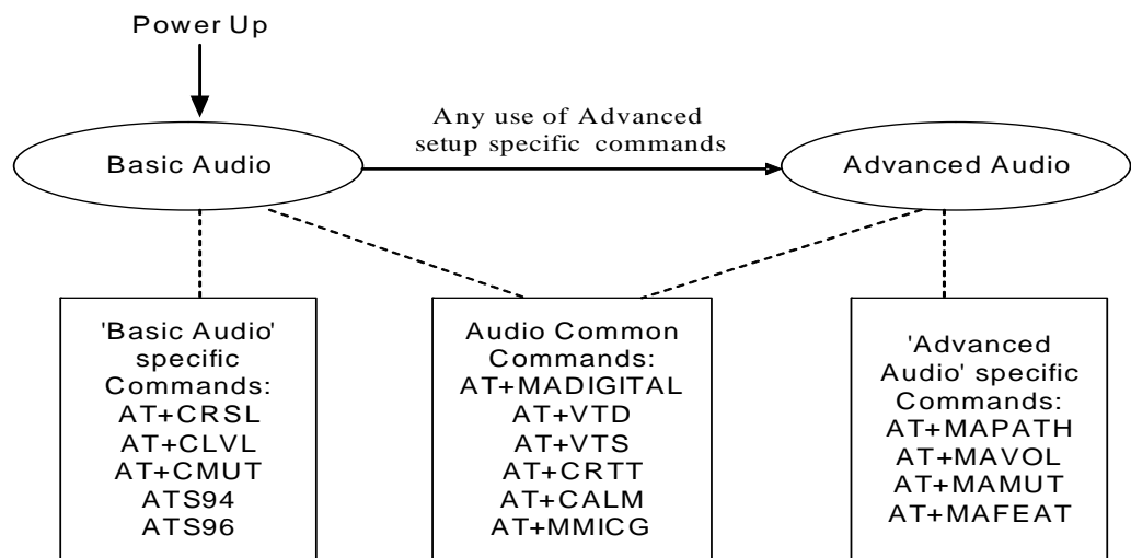
Figure 3-2: Audio Modes
