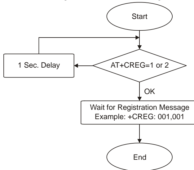
Figure 4-8: G24-L Network Connection
