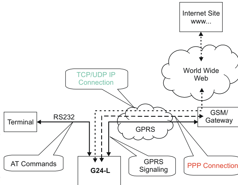
Figure 1-1: System Overview
